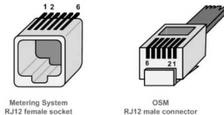
Figure 3: P1 Physical connector
